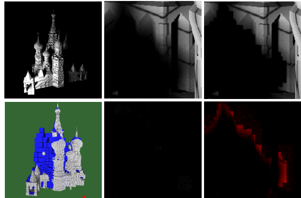
Figure 15: An example of artifacts in the area of soft shadows introduced by an acceleration technique which was not designed for extended light sources (middle: correct shadow, right: artifacts. Geometric model and octree on the left).
