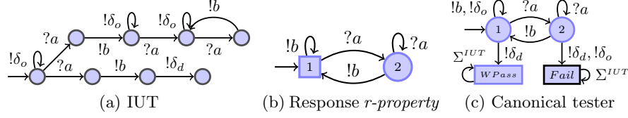
Fig. 6: Illustrating the usefulness of quiescence
