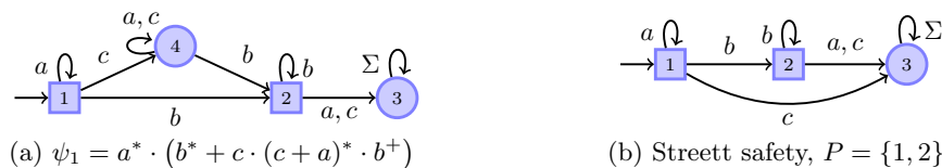
Fig. 3: DFA for \psi_1 and Streett for (A_f(\psi_1), A(\psi_1))
