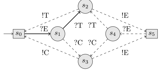
Figure 3. Specification \mathcal{S} of a coffee-machine
