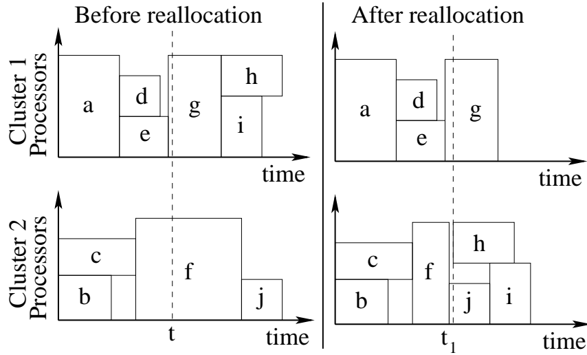
Figure 2: Example of reallocation between two clusters.
