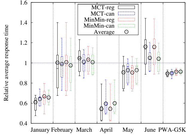
Figure 20: Relative average response time on heterogeneous non-dedicated platform.
