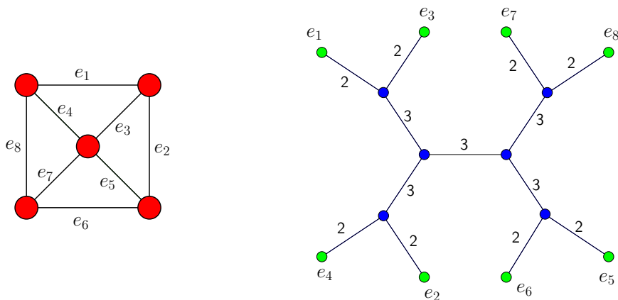
Figure 1: A graph and one of its branch decompositions, of width 3.
