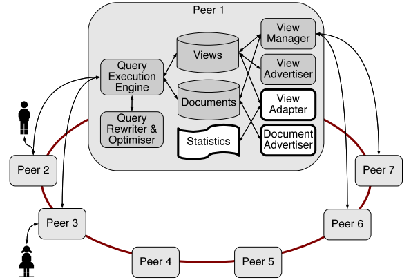
Figure 1: LiquidXML platform architecture.
