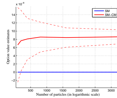
(f) Arithmetic Put with d = 5 assets
