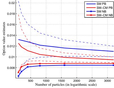
(c) Geometric Put with d = 4 assets
