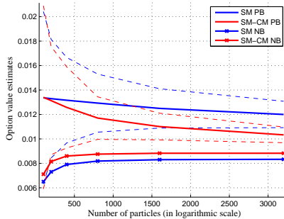
(e) Geometric Put with d = 5 assets
