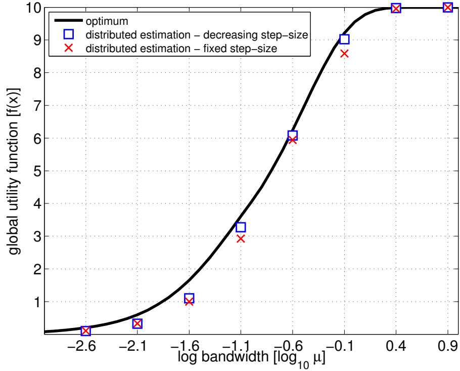
Figure 6: Theoretical maximum of the utility function vs utility of the rate allocation obtained with the distributed sub-gradient method for eight different bandwidth's values.
