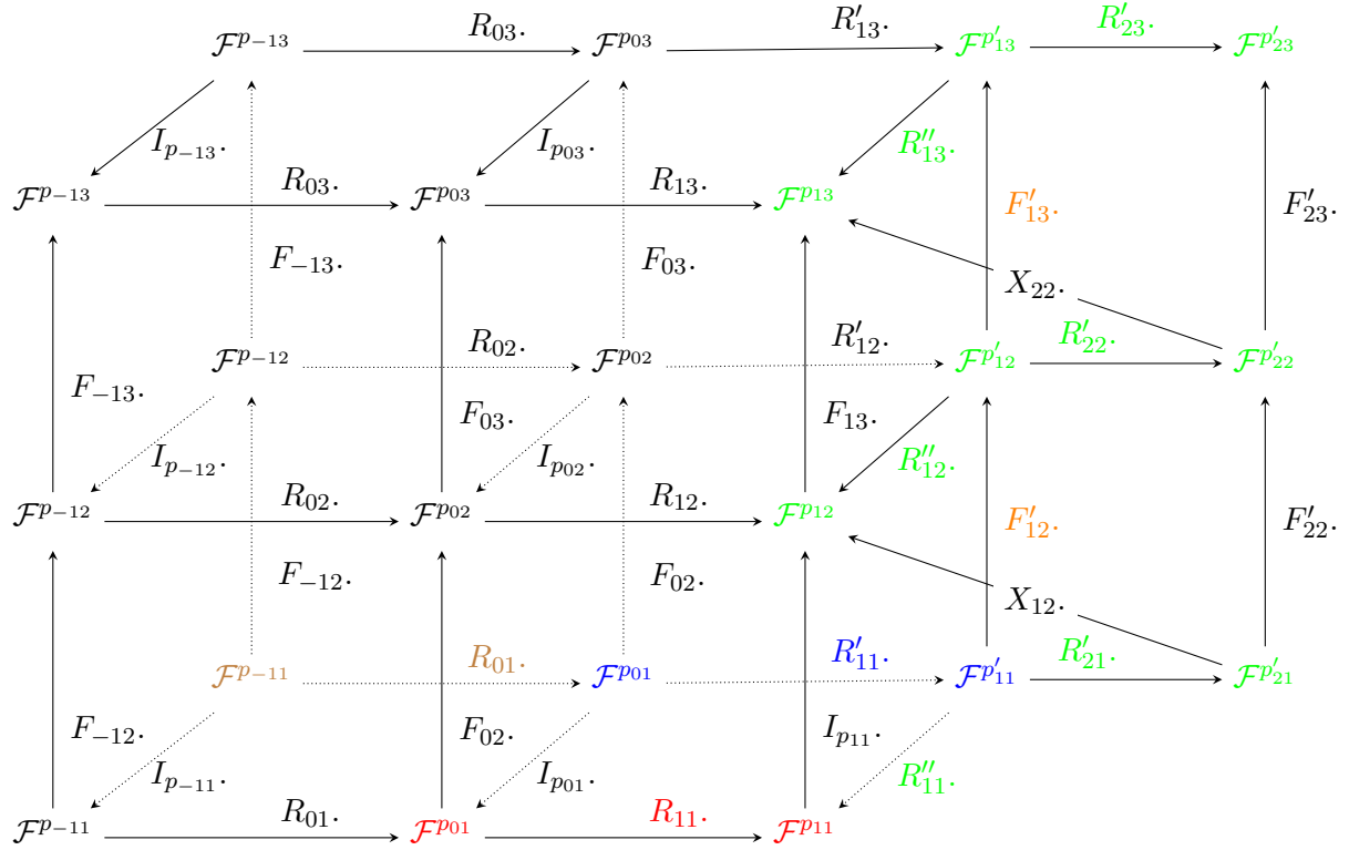
Figure 2.2: System equivalence based on the purity filtration
