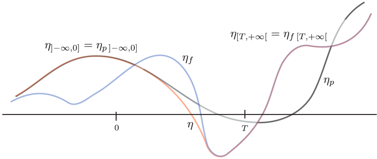
Figure 1.1: Controllability à la Willems
