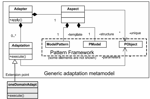
Figure 8: Adaptation Metamodel
