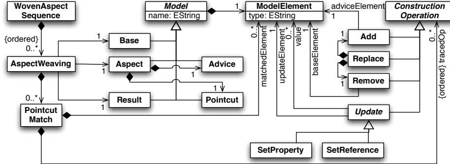
Fig. 2: Traceability Metamodel
