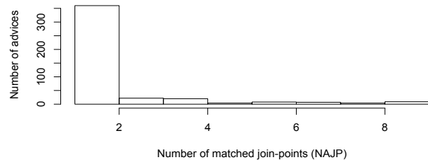
Figure 5. Histogram of NAJP frequency.
