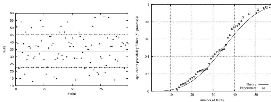
Figure 6. Number of faults leading to a crash for 100 experiments ( p = 50, r = 3 ) (left), Comparison of experimental numbers of faults with theoretical count (right)
