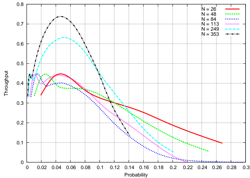
Figure 14: Throughput with slotted ALOHA protocol. Nodes are dispatched in network area of 100 \times 100m^2 according to Poisson distribution.
