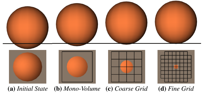
Figure 6: Intersection after one LCP solution of volume constraint stabilization for grids of different resolution. Increasing the multi-volume precision provides a more accurate linearization of the intersection volume gradients.
