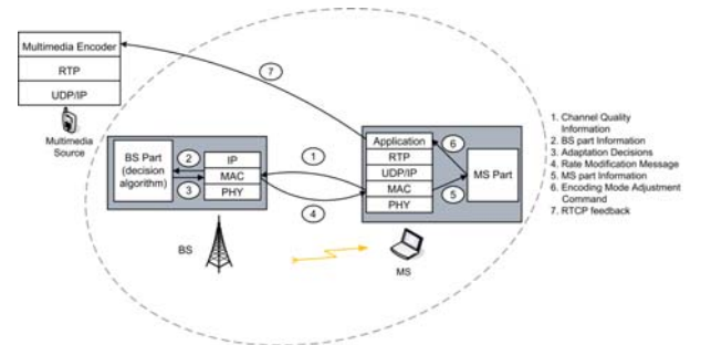
Fig. 1. The CLEMA mechanism for the downlink
