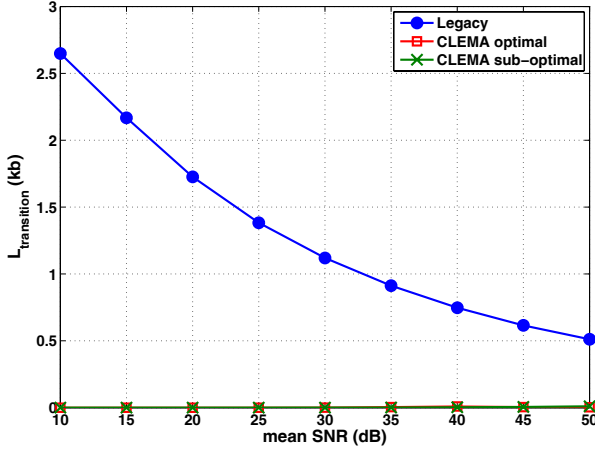
Fig. 5. L_{transition} vs. \bar{\gamma} (service rate per traffic frame c=10 symbols/5ms)
