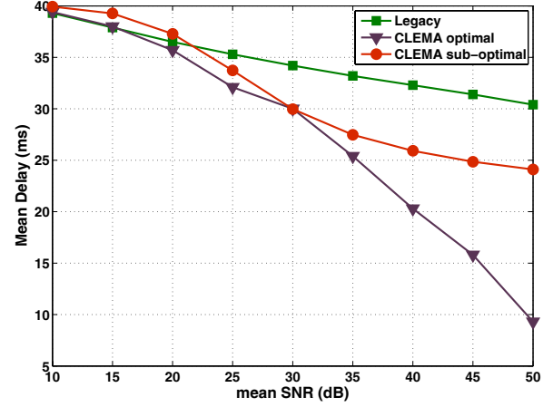
Fig. 6. Mean delay vs. \bar{\gamma}
