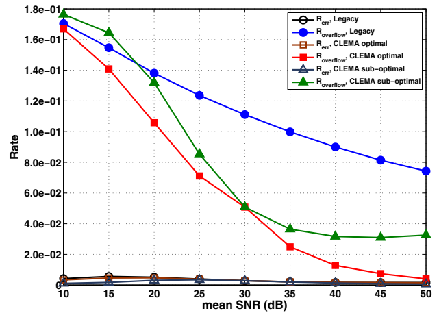
Fig. 4. R_{err} and R_{overflow} vs. \bar{\gamma}
