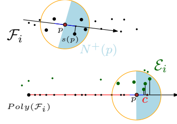
Figure 3: Illustration of feature recovery step. Top: procedure succ(p) that discovers the successor, s(p) , of a point p \in \mathcal{F}_i . Bottom: after smoothing the polyline Poly(\mathcal{F}_i) , we elongate it at each endpoint p using the detected extremity points \mathcal{E}_i .
