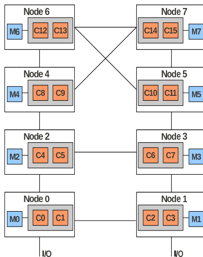
Figure 6: ccNUMA Platforms
