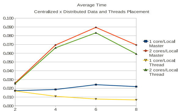
Figure 10: Average Time (s): Centralized x Distributed Data and Threads Placement
