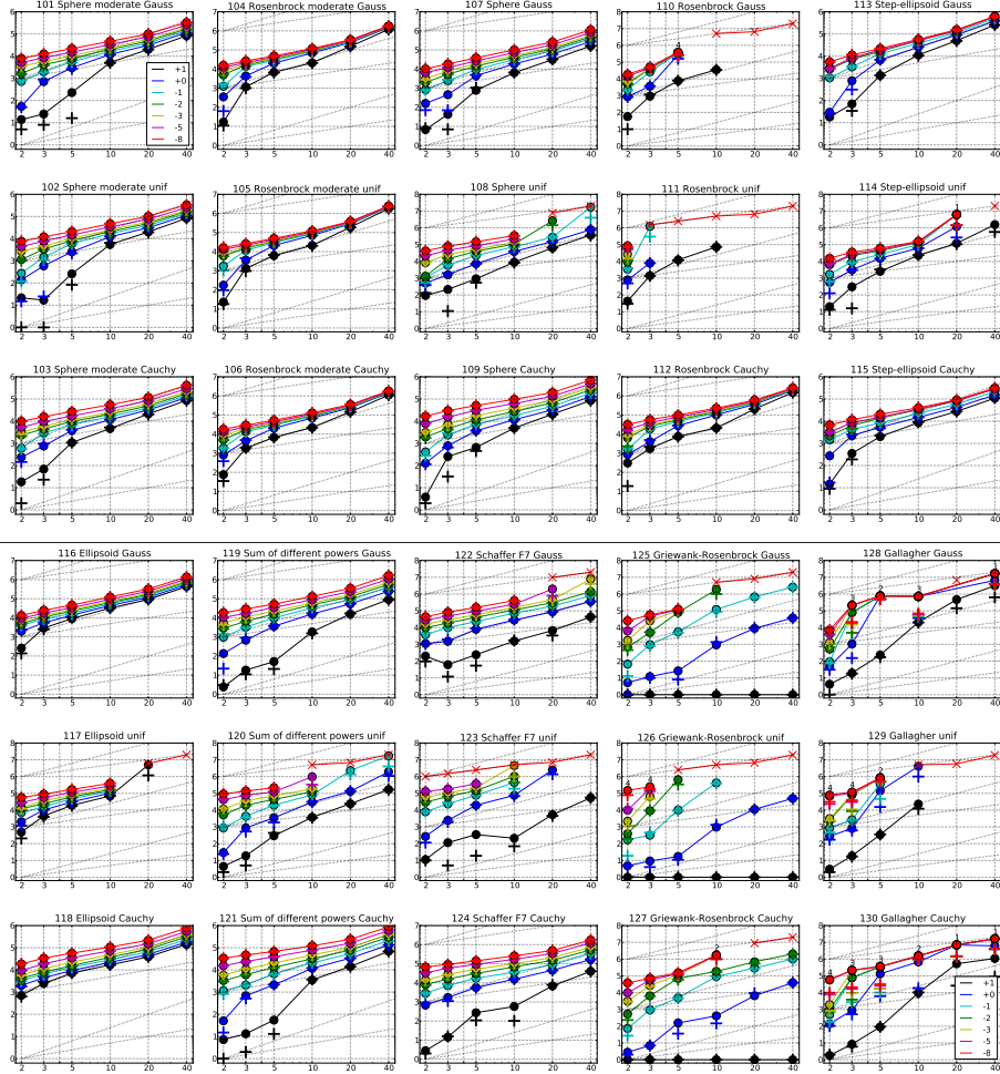
Figure 8: Expected Running Time (ERT, \bullet ) to reach f_{\text{opt}} + \Delta f and median number of function evaluations of successful trials (+) for CMA-ES with population size 128 times standard, shown for \Delta f = 10, 1, 10^{-1}, 10^{-2}, 10^{-3}, 10^{-5}, 10^{-8} (the exponent is given in the legend of f_{101} and f_{130} ) versus dimension in log-log presentation. The ERT(\Delta f) equals to \#FEs(\Delta f) divided by the number of successful trials, where a trial is successful if f_{\text{opt}} + \Delta f was surpassed during the trial. The \#FEs(\Delta f) are the total number of function evaluations while f_{\text{opt}} + \Delta f was not surpassed during the trial from all respective trials (successful and unsuccessful), and f_{\text{opt}} denotes the optimal function value. Crosses ( \times ) indicate the total number of function evaluations \#FEs(-\infty) . Numbers above ERT-symbols indicate the number of successful trials. Annotated numbers on the ordinate are decimal logarithms. Additional grid lines show linear and quadratic scaling.
