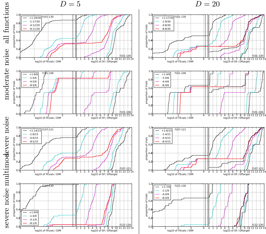
Figure 5: Empirical cumulative distribution functions (ECDFs) for CMA-ES with standard population size, plotting the fraction of trials versus running time (left subplots) or versus \Delta f (right subplots). The thick red line represents the best achieved results. Left subplots: ECDF of the running time (number of function evaluations), divided by search space dimension D , to fall below f_{\text{opt}} + \Delta f with \Delta f = 10^k , where k is the first value in the legend. Right subplots: ECDF of the best achieved \Delta f divided by 10^k (upper left lines in continuation of the left subplot), and best achieved \Delta f divided by 10^{-8} for running times of D, 10D, 100D \dots function evaluations (from right to left cycling black-cyan-magenta). The legends indicate the number of functions that were solved in at least one trial. FEvals denotes number of function evaluations, D and DIM denote search space dimension, and \Delta f and Df denote the difference to the optimal function value.
