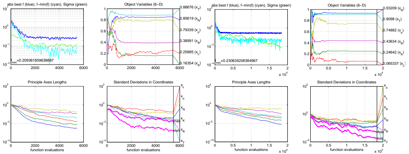
Figure 11: Standard output of the CMA-ES for two independent runs with a population size of \lambda = 48 . Left: first run with 5424 function evaluations; Right: second run with 18226 function evaluations. The reason for the early stop of the run shown on the left was the meeting of the stopping criterion optimal value found . However, we believe that this was caused by a numerical error as the re-evaluation of the corresponding search point gave an objective value of 0.4116519215632899.
