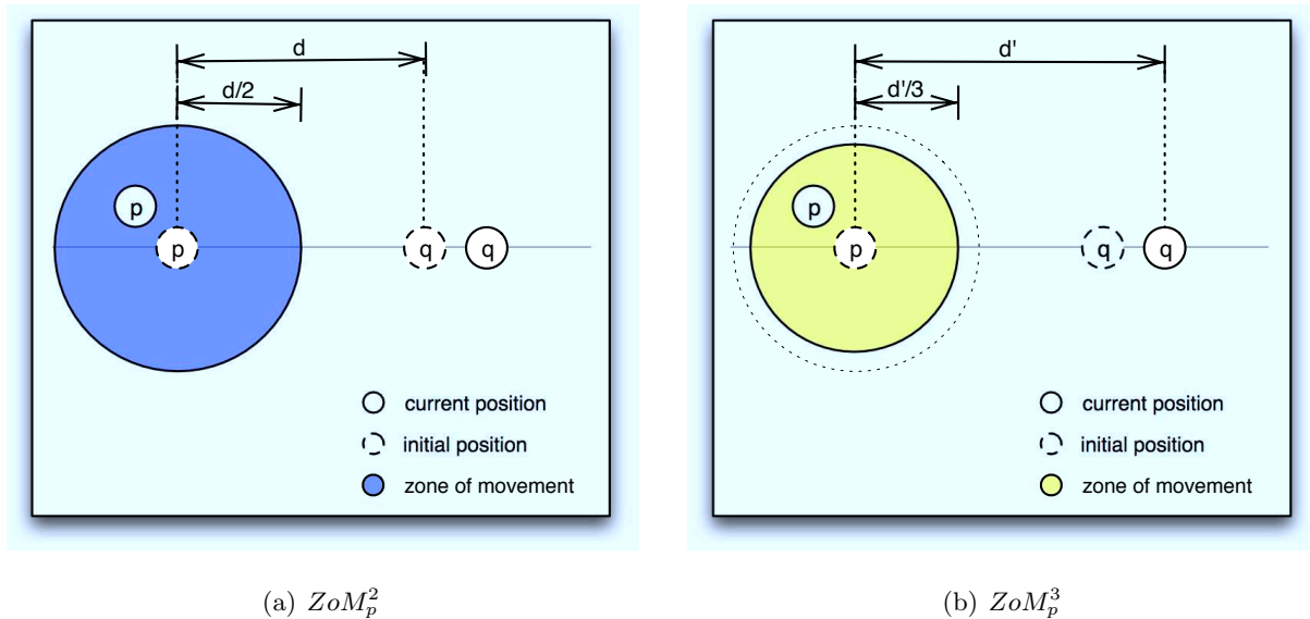
Figure 1: Example zones of movement: The network is formed of two robots: p and q . d is the distance between the initial positions of p and q (dashed circles), d' is the distance between the initial position of p and the current position of q . The diameter of ZoM_p^2 (blue) is d/2 and that of ZoM_p^3 (yellow) is d'/3 .
