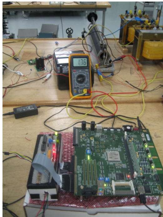
Figure 9. Picture of the set-up including the FPGA device in the foreground and the Ćuk converter in the background.
