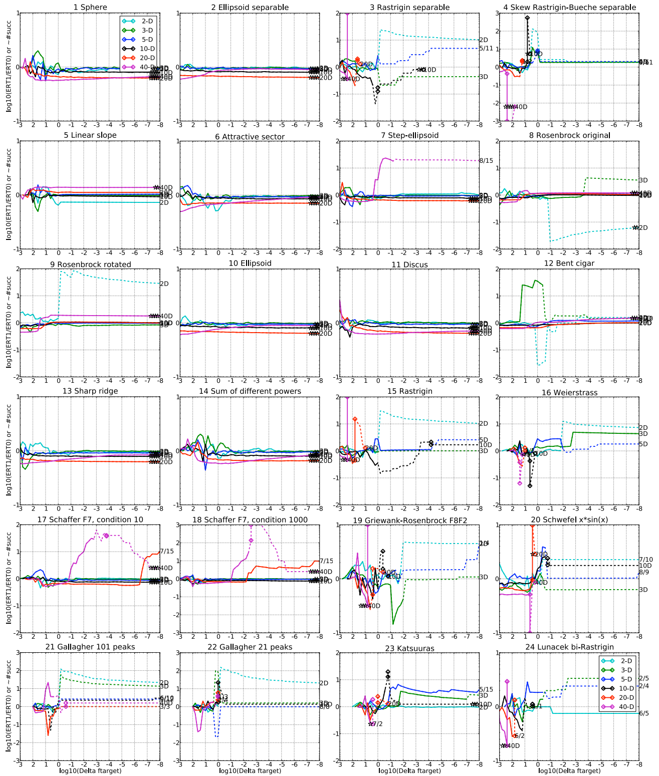
Figure 1: ERT ratio of PM-AdapSS-DE divided by Uniform-DE versus \log_{10}(\Delta f) for f_1 – f_{24} in 2 , 3 , 5 , 10 , 20 , 40 -D. Ratios < 10^0 indicate an advantage of PM-AdapSS-DE, smaller values are always better. The line gets dashed when for any algorithm the ERT exceeds thrice the median of the trial-wise overall number of f -evaluations for the same algorithm on this function. Symbols indicate the best achieved \Delta f -value of one algorithm (ERT gets undefined to the right). The dashed line continues as the fraction of successful trials of the other algorithm, where 0 means 0% and the y-axis limits mean 100%, values below zero for PM-AdapSS-DE. The line ends when no algorithm reaches \Delta f anymore. The number of successful trials is given, only if it was in \{1 \dots 9\} for PM-AdapSS-DE (1st number) and non-zero for Uniform-DE (2nd number). Results are significant with p = 0.05 for one star and p = 10^{-\#*} otherwise, with Bonferroni correction within each figure.
