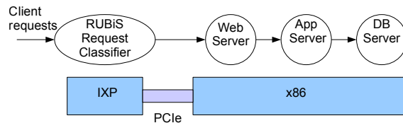
Figure 1: RUBiS Components on IXP and x86 systems and their Interactions on Receive Path.
