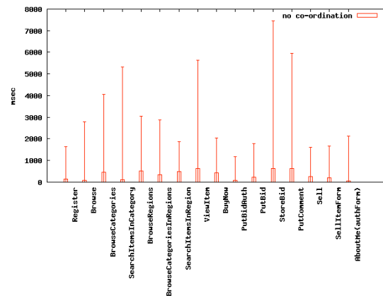
Figure 2: RUBiS: Variation in minimum-maximum response latencies.
