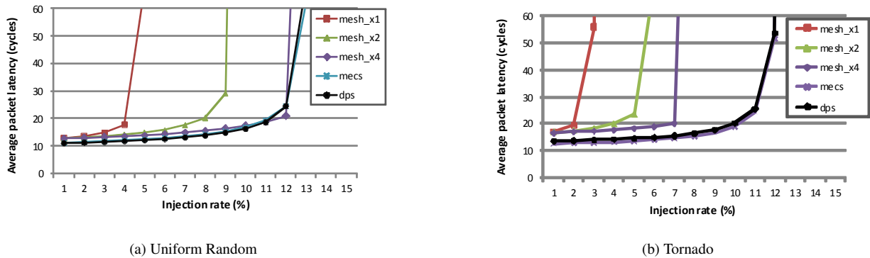
Figure 4. Latency and throughput on synthetic traffic.
