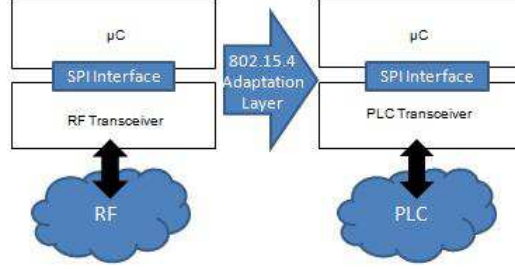
Figure 4: Emulation of a classic RF transceiver by a PLC transceiver through an enhanced SPI interface
