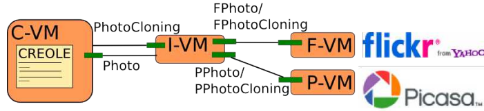
Figure 3: Flickr-Picasa Integration
