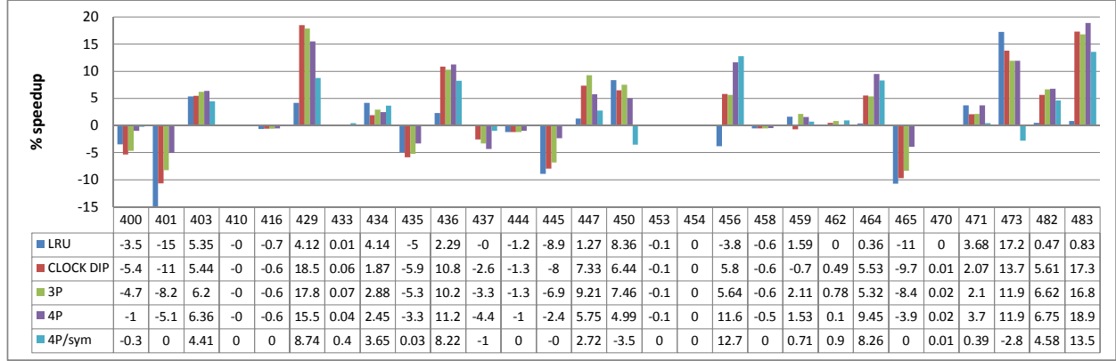
Figure 2: Percentage of speedup on a 4MB 16-way L3 cache shared by 4 threads. The baseline performance for each benchmark is the symmetric performance under LRU.
