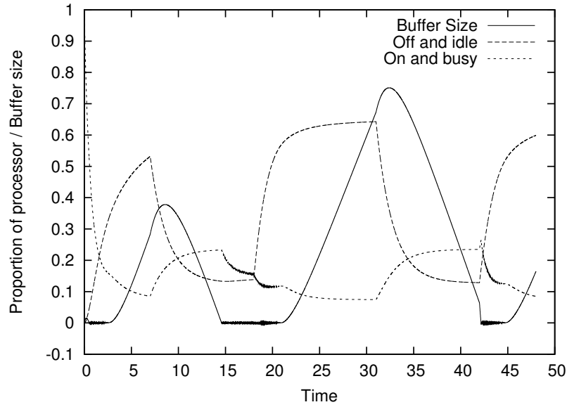
Figure 3: Limit dynamics for volunteer computing under day and night availability.
