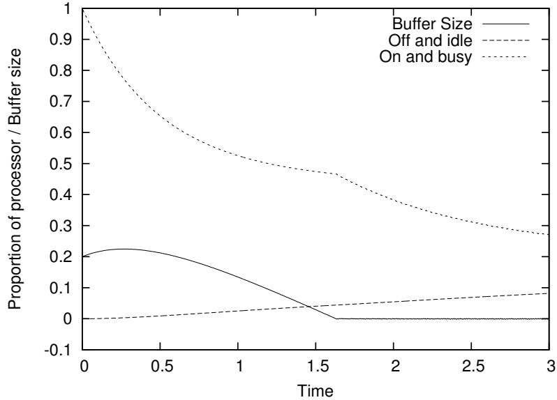
Figure 2: Limit dynamics of a volunteer computing system. A non-differentiable point occurs when the buffer becomes empty.
