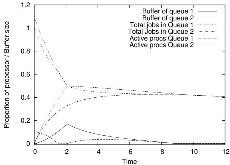
Figure 4: Join the shortest queue for volunteer computing
