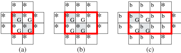
Figure 3. Local sub-problems tackled in the proof of Theorem 1.
