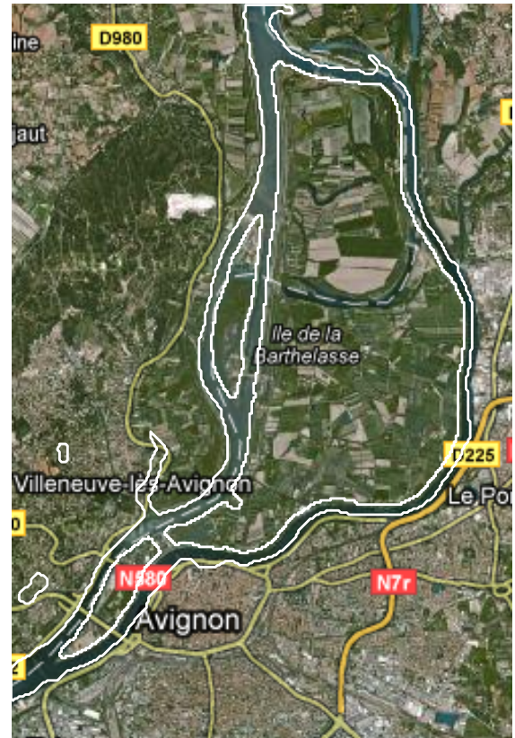
Figure 4: River network segmentation from a colour image using the new algorithm. Flow conservation is satisfied at junctions, illustrated by a significant change of width, and along branches, as illustrated by a slow change of width. (©2010 Google - Imagery ©2010 TerraMetrics, Map data ©2010 Tele Atlas.)
