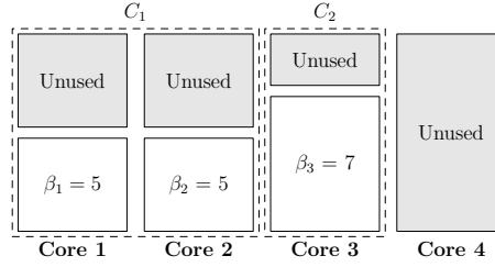
Fig. 1: An example of a CPU emulation problem. Here: N = 4 , \alpha_1 = \alpha_2 = \alpha_3 = \alpha_4 = 10 , M = 2 , C_1 = \{1, 2\} , C_2 = \{3\} , \beta_1 = \beta_2 = 5 , \beta_3 = 7 , \beta_4 = 0 .
