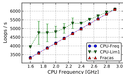
Figure 5: Sleep benchmark
