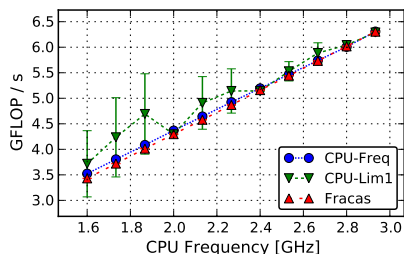
Figure 4: Linpack benchmark
