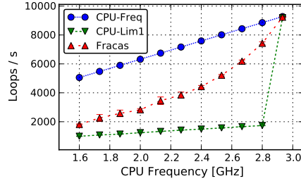
Figure 7: Threads benchmark
