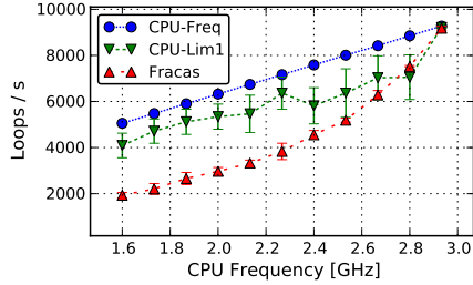
Figure 6: Processes benchmark
