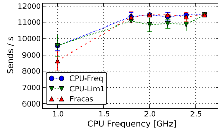
Figure 9: UDP benchmark (on Chti cluster)
