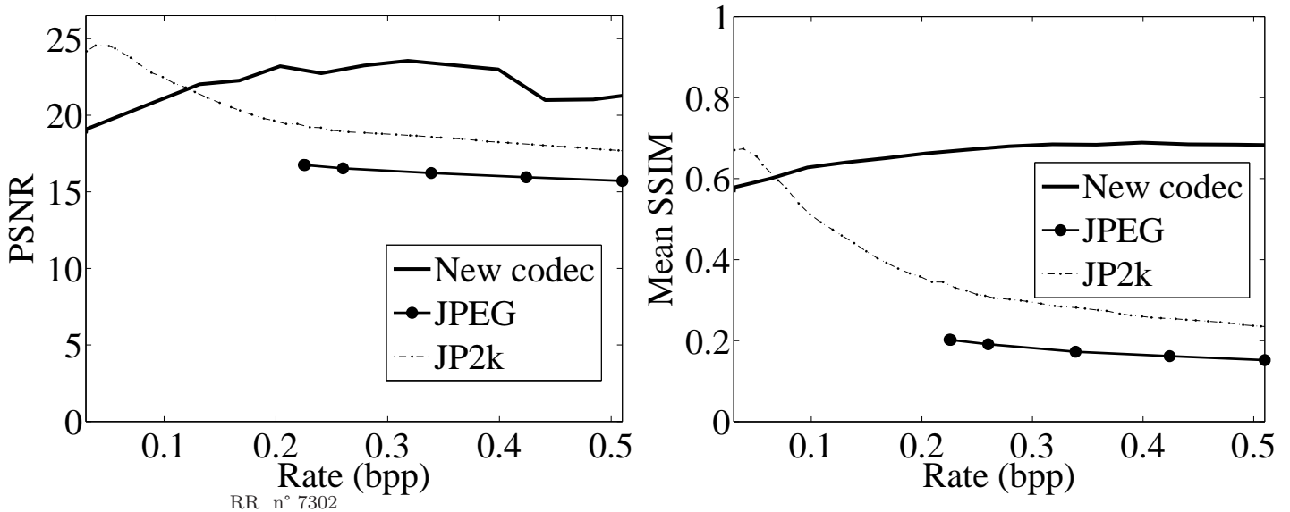
Figure 23: Rate/Quality behavior: quantitative comparison between our new codec, JPEG, and JPEG2000 using two different quality measures.
