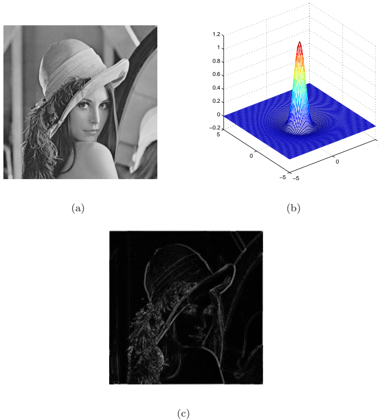
Figure 10: Behavior of the dog filter when applied to Lena with biologically plausible parameters. (a): the classical test image Lena. (b): the dog filter with parameters \alpha = 3 and w_c = w_s = 1 and \sigma = 0.5 . (c): the absolute value of the image resulting from the convolution of Lena with the filter in (b).
