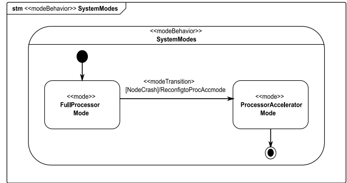
Fig. 5: Mode specification with a FSM in MARTE.
