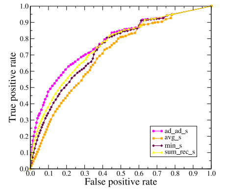
Figure 10: ROC curves for features related to group sizes.
