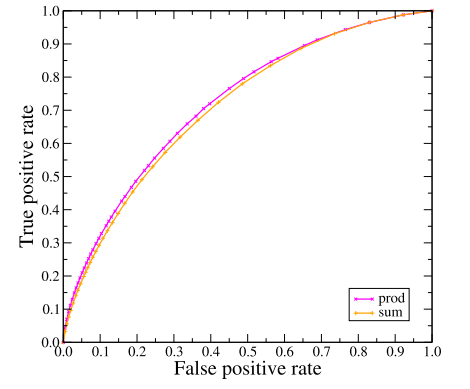
Figure 4: ROC curves for features related to the number of group memberships of users.
