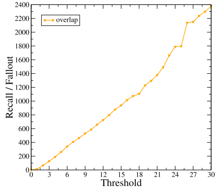
Figure 6: The recall/fallout curve for the overlap feature.
