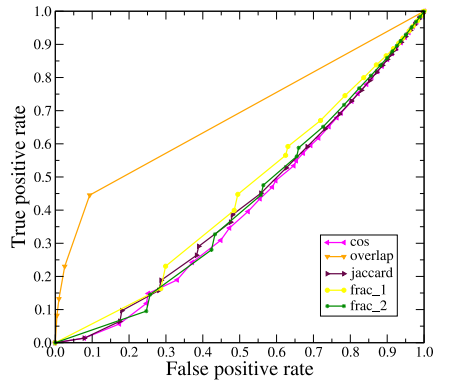
Figure 7: ROC curves for features related to similarity of group memberships.
