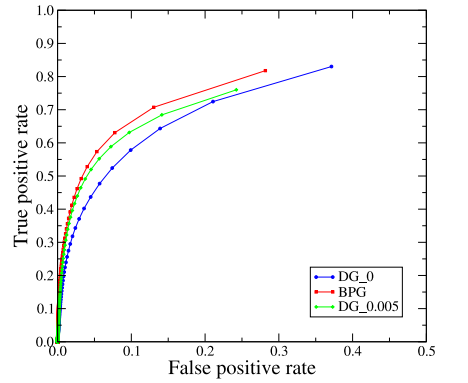
Figure 25: ROC curves for the rooted_pagerank feature (friends).
