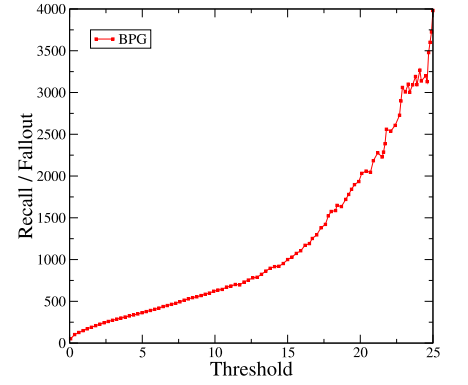
Figure 22: Recall/fallout for the common_neighbors feature.
