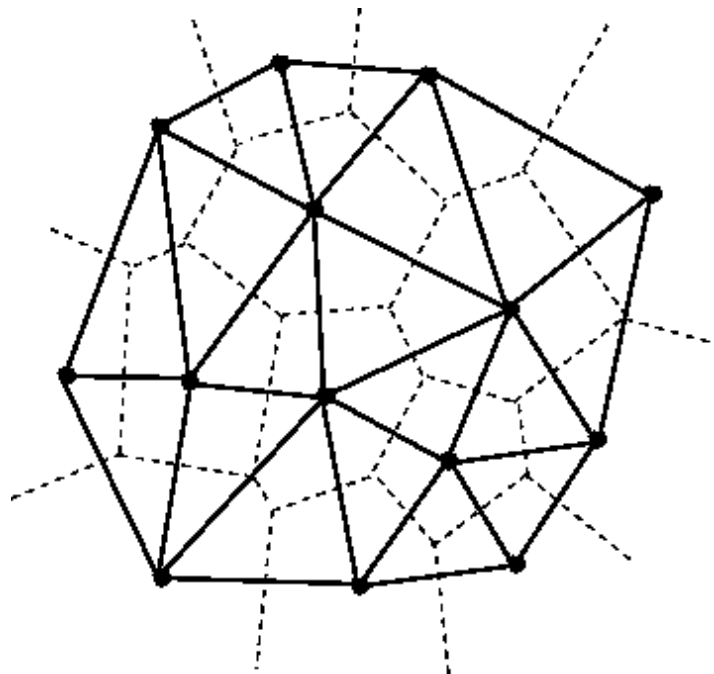
Figure 3: Delaunay Triangulation
