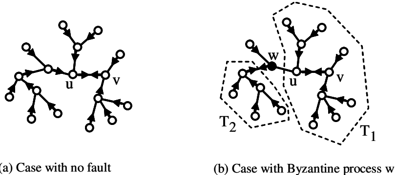
Figure 1: Tree orientation
