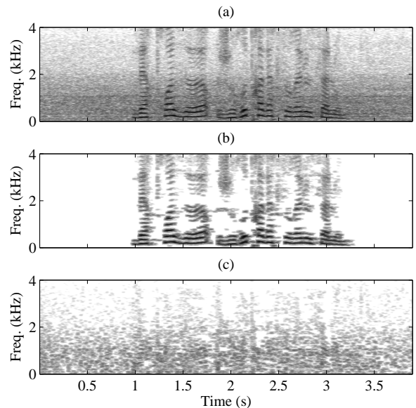
Figure 4: Speech spectrograms. (a) Noisy speech; (b) Noisy speech enhanced by RFSNR technique; (c) Musical noise successfully removed using the RFSNR technique.
