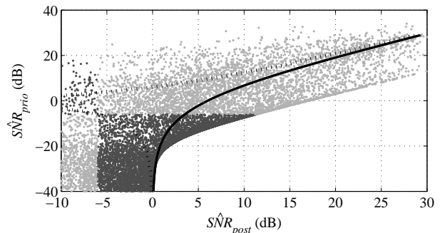
Figure 3: Separation of the features defined by S\hat{N}R_{prio} of DD approach versus S\hat{N}R_{post} . The RFSNR approach leads to a separation in 4 quadrants using 2 thresholds on S\hat{N}R_{post} and S\hat{N}R_{prio} .
