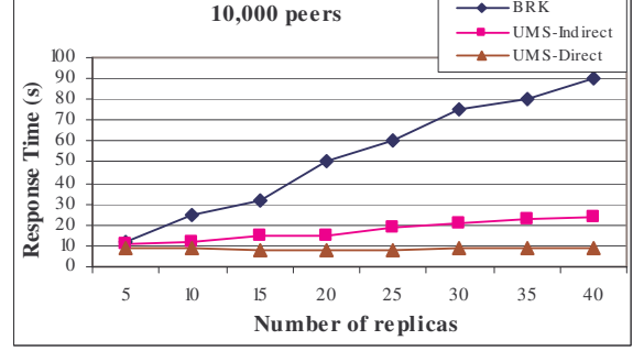
Figure 9. Response time vs. number of replicas
