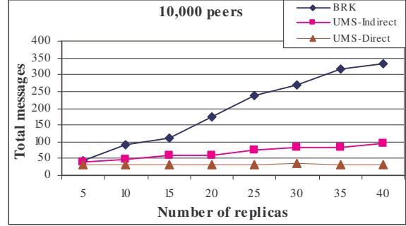
Figure 10. Communication cost vs. number of replicas
