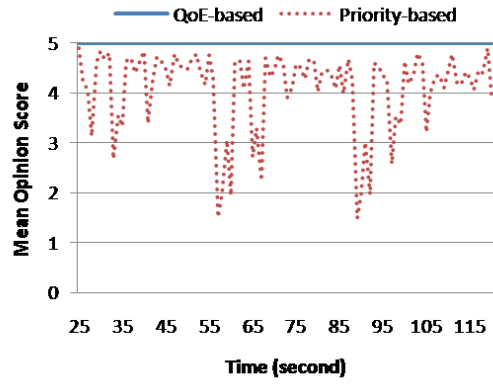
FIG. 8 – Quality experienced by MN under critical condition
