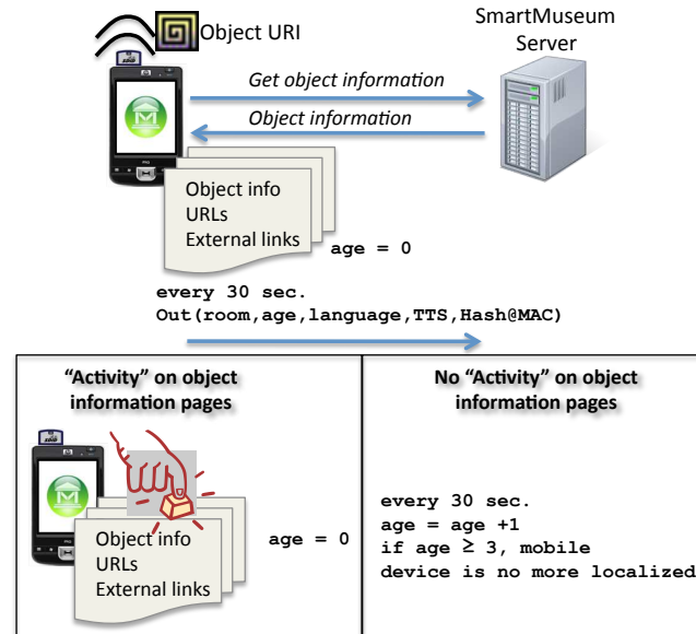
Figure 3: Location mechanism
