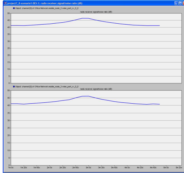
Figure 9: SNR values of two neighbor nodes
