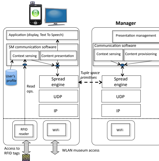
Figure 2: System architecture
