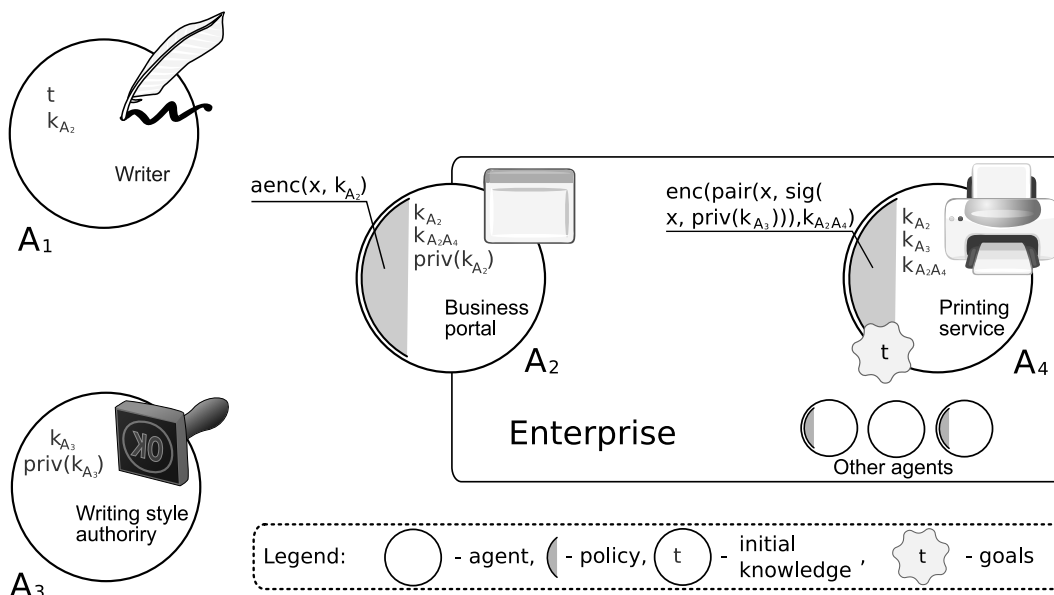
Figure 2: Illustration for agents cooperation example
