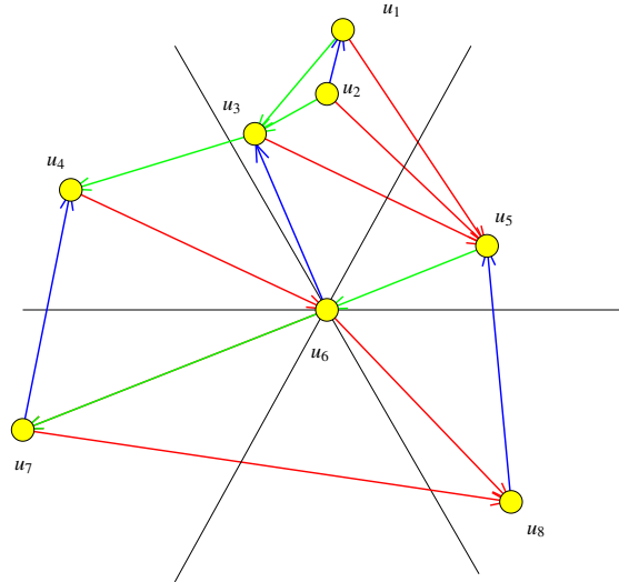
Fig. 1: An example of \frac{1}{2}\Theta_6 .
