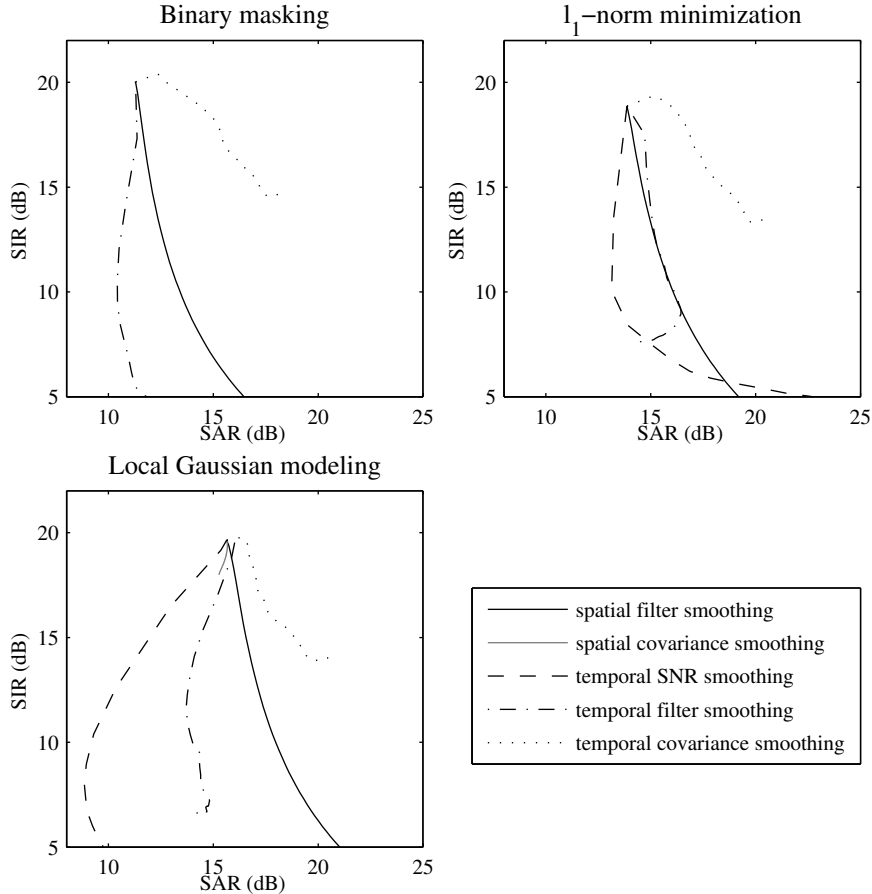
Figure 1: Average tradeoff between SAR and SIR achieved by each separation algorithm and each smoothing technique.
