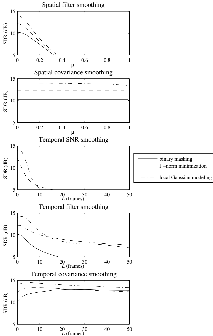
Figure 2: Average SDR achieved by each separation algorithm and each smoothing technique as a function of the smoothing parameter.
