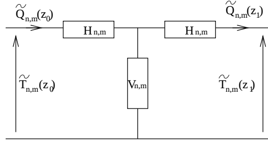
Figure 2: Network representation for a homogeneous layer : transformed temperature and heat flux are equivalent to voltage and current respectively.
